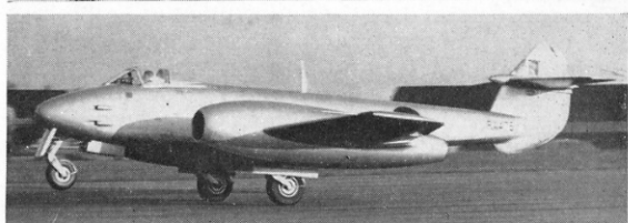
Above, top: E.E.455 "Britannia" or the "Yellow Peril", achieved 603 m.p.h. when attempting the Air Speed Record in 1945. Above, bottom: R.A.476 broke the Turnhouse, Scotland-Bovingdon, Hertfordshire record. Below: E.E.549 which broke the World Air Speed Record in 1946 with a speed of 616 m.p.h. The Meteor now stands outside R.A.F. Innsworth. (Photos: the author)
