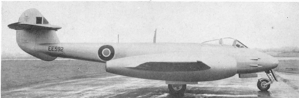
Side, rear and underside flying view of a typical Meteor F. Mk. 4 powered by Rolls-Royce Derwent 5 turbo-jets. E.E.592 was a type G.41F Gloster-built aircraft. (Photos: Ministry of Defence)
