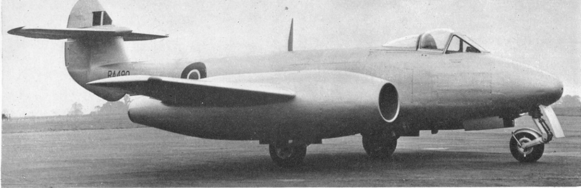
Another RA-serialised Meteor to be used as an engine test-bed was 490, shown with Metro-Vick Beryl axial-flow engines. These were later replaced by non-standard Rolls-Royce Nenes fitted with jet deflection units. As a STOL aircraft the Meteor was the forebear of the Hawker Siddeley Kestrel. The airframe was drastically modified; major modifications being the F. Mk. 8 tail assembly and the end-plate fins on the tailplane. (Photo: Hawker Siddeley Aviation Ltd.)
