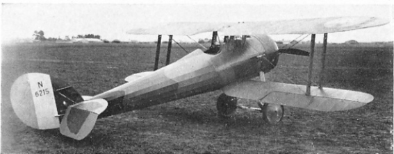
Late production Nieuport 28, serial number 6215, showing correct form of U.S. tail striping. (Photo: U.S. National Archives)
