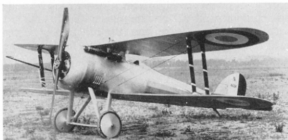
Modified Nieuport 28 prototype, still with single-unit interplane struts but dihedral added to top wing by shortening centre section struts and bringing wing down to fuselage. (Photo: Nieuport)
