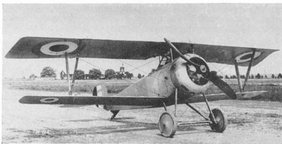
Above, left: The most famous fighting ancestor of the Nieuport 28—the Model 17. (Photo: Signal Corps, U.S. Army). Right: The beginning of the Nieuport 28—a modified Model 24 with 160-h.p. Gnome engine and centre section struts altered to permit mounting of single Vickers machine gun outboard of the struts. New tail shape had appeared on Model 23. (Photo: Nieuport)
