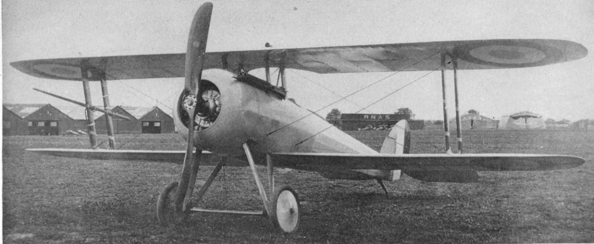
Prototype Nieuport 28 showing absence of dihedral on upper wing.
