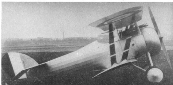
Left: Further evolution of the Model 28—a modified 24 with enlarged two-spar lower wing that increased the total wing area to eighteen square metres from the fifteen of the standard Model 24. Right: Original prototype of the Nieuport 28 with single machine gun and unique one-piece interplane struts. (Photos: Nieuport)
