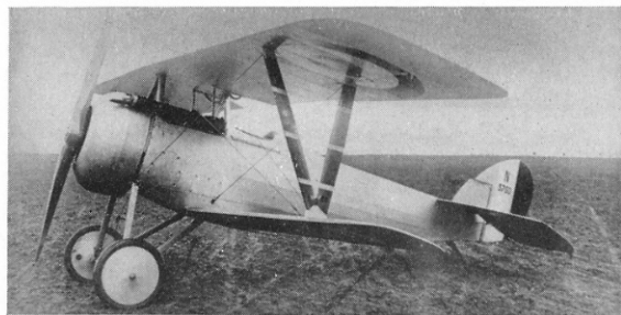
Above, left: The most famous fighting ancestor of the Nieuport 28—the Model 17. (Photo: Signal Corps, U.S. Army). Right: The beginning of the Nieuport 28—a modified Model 24 with 160-h.p. Gnome engine and centre section struts altered to permit mounting of single Vickers machine gun outboard of the struts. New tail shape had appeared on Model 23. (Photo: Nieuport)
