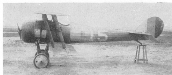
Nieuport 28 of 94th Pursuit Squadron forced down in enemy territory. Compare rudder striping with later models. Below: A different view of the same machine. Apparently the Germans made a very hasty assembly for inspection purposes after bringing the machine to the rear area for the top wing is rigged with no dihedral while the lower wing droops. (Photos: Official German)
