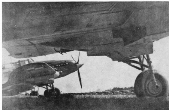
Polish Air Force Il-2m3s; note underwing detail.
