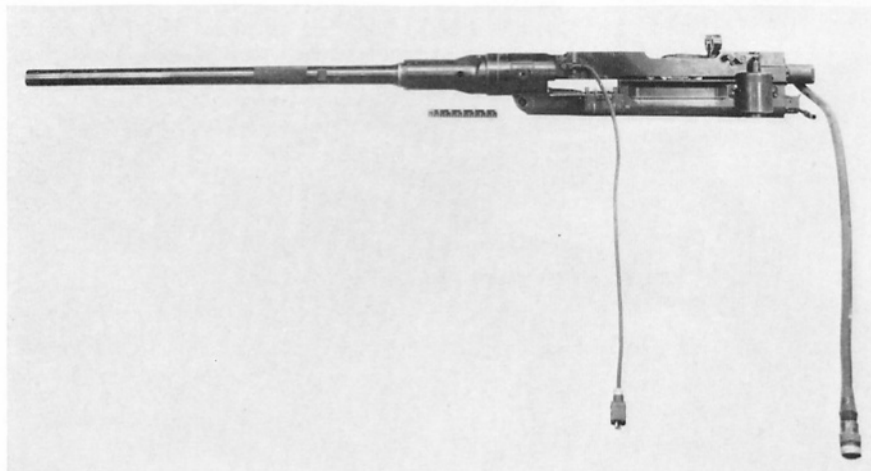
The slim belt-fed Mauser MG 151 20 mm. cannon armed the later versions of the Ju 88 night fighter series. The scale indicator is six inches long. (Photo: Crown copyright)
