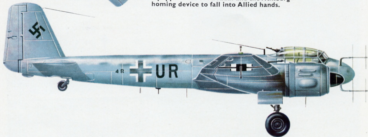
JUNKERS JU 88G-1, 4R + UR, of 7th Staffel, Nachtjagdgeschwader 2. In the early hours of 13th July, 1944 this aircraft landed in error at Woodbridge, Essex, U.K. after flying a reciprocal compass course. It was the first intact example of an aircraft equipped with SN-2 radar and the Flensburg homing device to fall into Allied hands.
