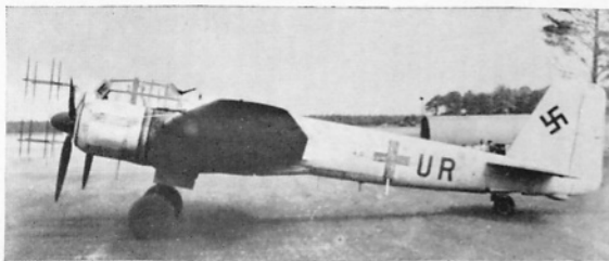
4R+UR, a Ju 88G-1 of 7/NJG 2, pictured after its inadvertent landing at Woodbridge in Essex during the early hours of 13th July, 1944. This aircraft furnished the R.A.F. with vitally important information about the SN-2 radar installation and the Flensburg homing device.
