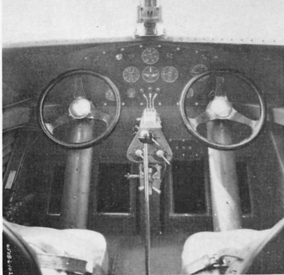
The pilot's cockpit of the Ford was simple and direct. The "Johnson Bar" in the centre was the hand-operated brake control. Instruments for the wing engines were mounted outside on an engine nacelle strut. (Photo: Ford Archives)
