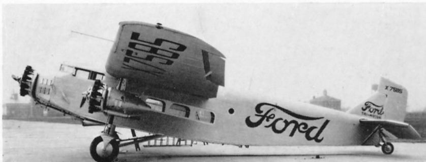
The single 9-A was a 4-AT-E with Pratt & Whitney Wasp Junior engines, serial numbers 1, 3 and 4. (Photo: Ford Archives)
